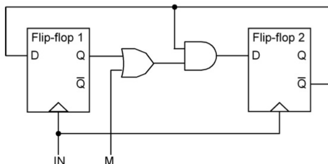
Figure 15. Modulo-2/3 dual-modulus prescaler circuit [7].
