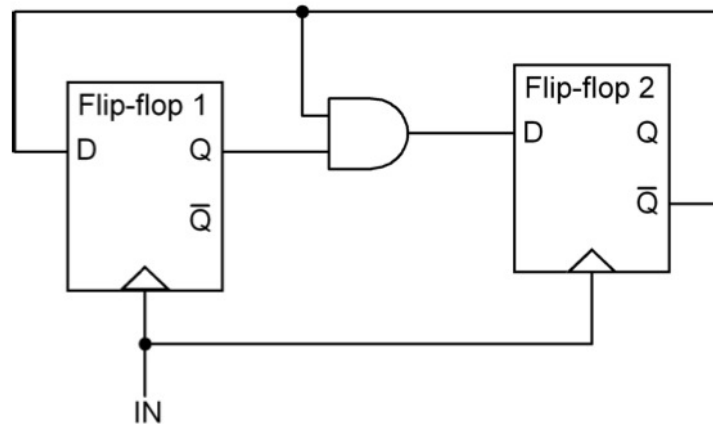
Figure 13. 1:3 prescaler [7].
