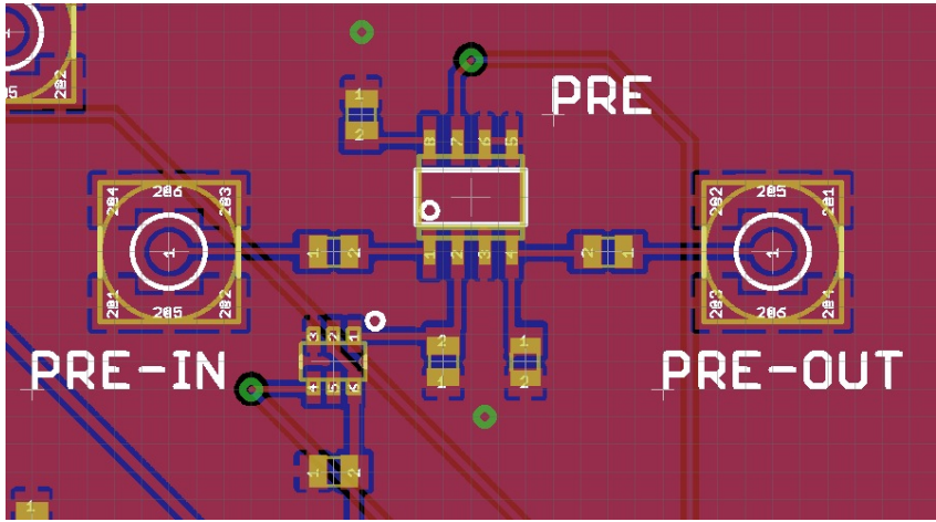
Figure 43. PCB layout for MC12080 prescaler.
