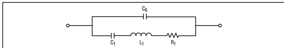
Figure 7. Equivalent circuit of the crystal [5].
