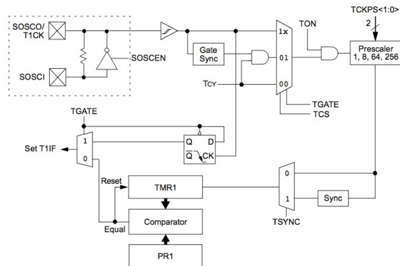
Figure 32. 16-bit Timer1 module block diagram.
