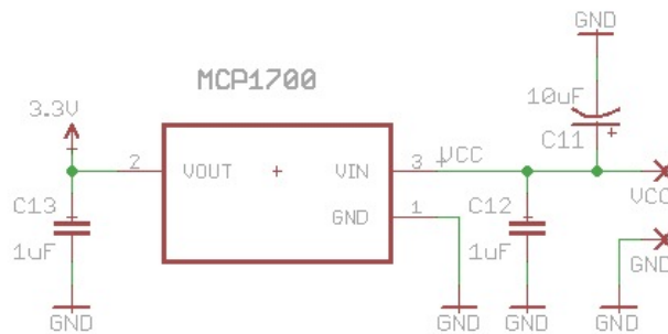
Figure 29. Power supply section schematic.
